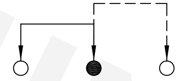
SCHEMATIC (NON-SHORTING)
